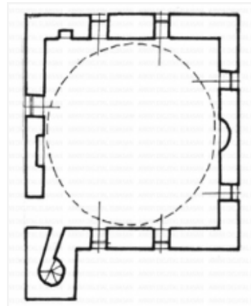
Figure 23: Mosque floor plan. (Meksi, 2012)
