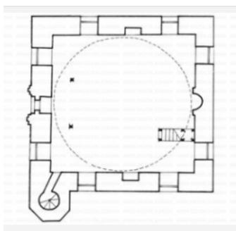
Figure 7: Mosque floor plan. (Meksi, 2012)
