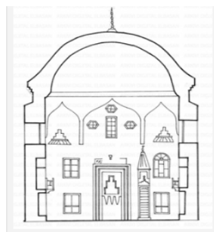
Figure 8: Mosque section. (Elbasan Digital archive's)
